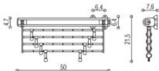
side view detail 側面図 fixed with shelf - support 棚板に取付
