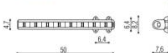
side view detail 側面図 fixed with shelf- support 棚板に取付
