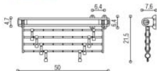
side view detail 側面図 fixed with shell - support 棚板に取付
